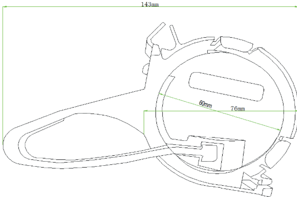
Technical drawing of ACC tension clamp
